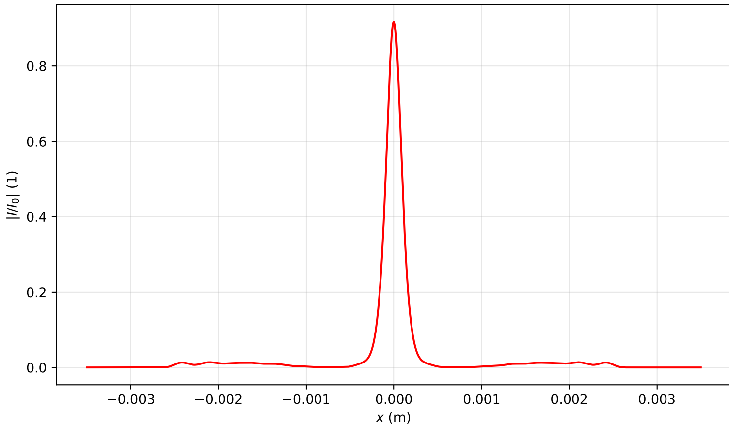
Intensity profile I(x, y = 0, z = 2.070)/I_0 , P_{in}=9.0P_{cr} , artificial time
